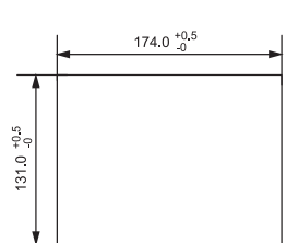
Panel cutout
