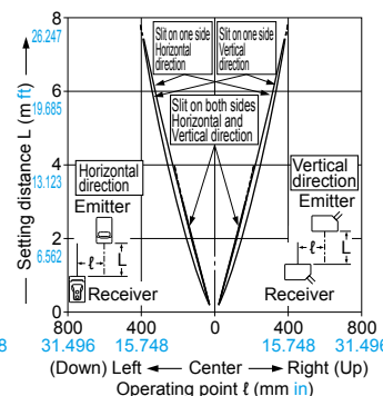
Parallel deviation with rectangular slit masks (2 × 6 mm 0.079 × 0.236 in)
